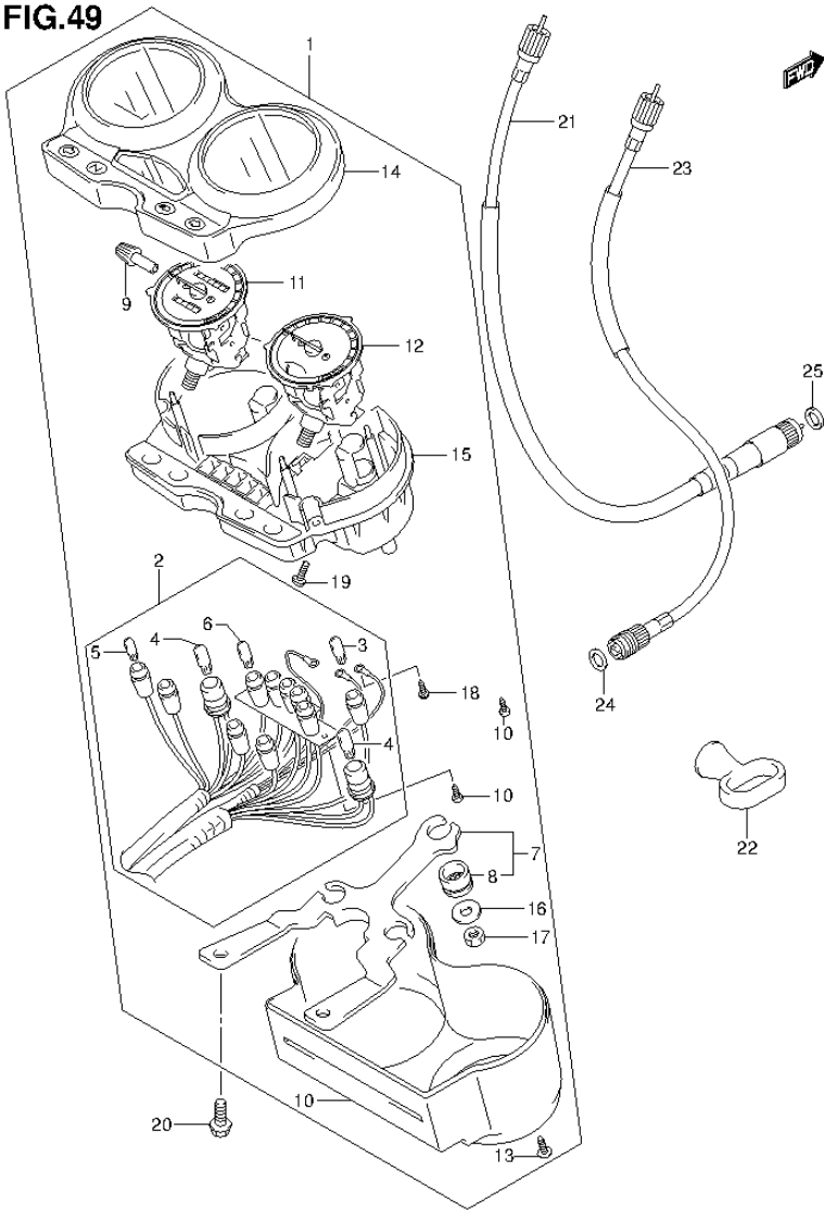
FIG.49 (1-F-6) SPEEDOMETER (EN125HUZL3 P71)
