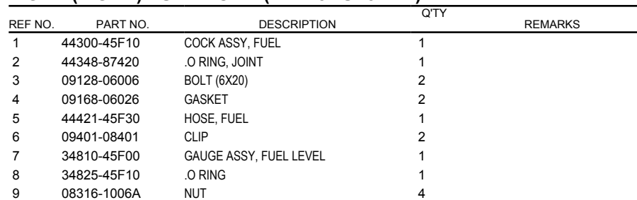
FIG.71 (1-G-14) FUEL COCK (EN125HUL3 P71)
